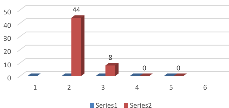
Figure 9: Students Feedback
